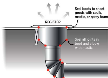
Above: Paint mastic (a thick, gooey substance) onto the duct seams and joints. (Photo source: Habitat for Humanity, Lakeland, FL)
