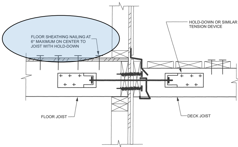
FIGURE R507.9.2(1) DECK ATTACHMENT FOR LATERAL LOADS
